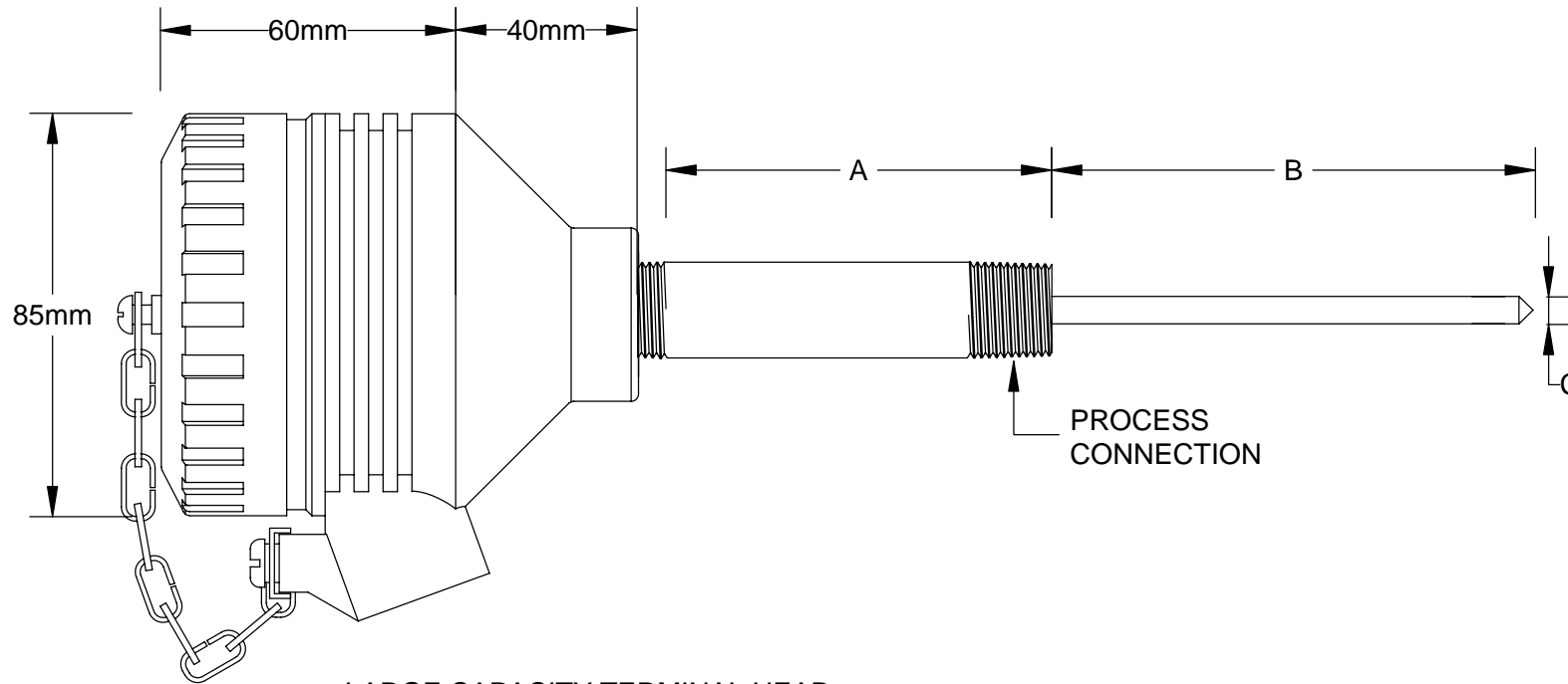
LARGE CAPACITY TERMINAL HEAD INTERNAL - 62mm Ø x 36mm HIGH Suitable for 33mm and 40mm centres
